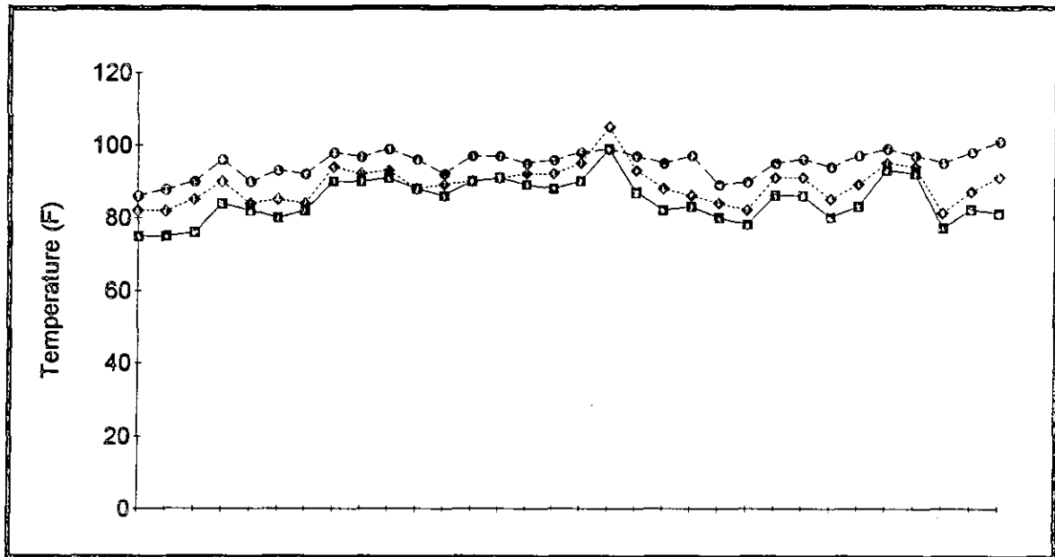
Fig. 1 Relative cloacal (circles), air temperature (diamonds) and basking surface temperatures (squares) for Crotaphytus collaris (n=32).
