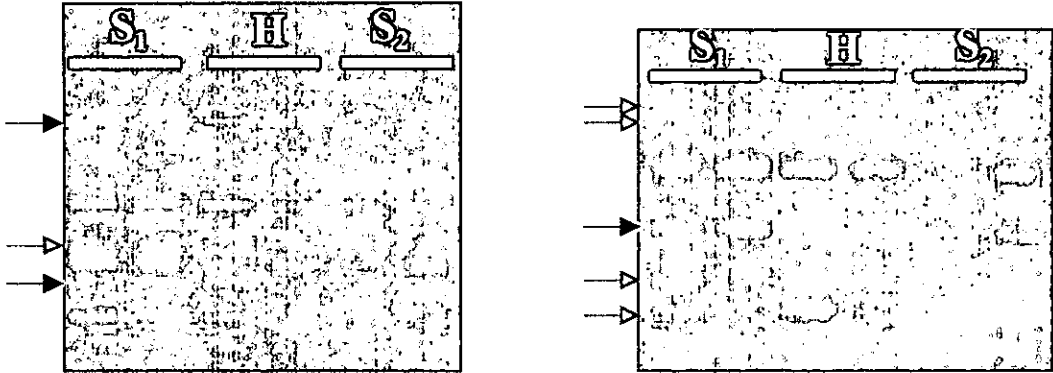
Figure 1. Portions of RAPD gels showing candidate loci (arrows) that distinguish Solidago sciaphila (two different populations: S 1 , S 2 ), from S. hispida (H). Black arrows indicate loci that differentiate the two species, while gray arrows indicate loci that may be unique to particular populations.
