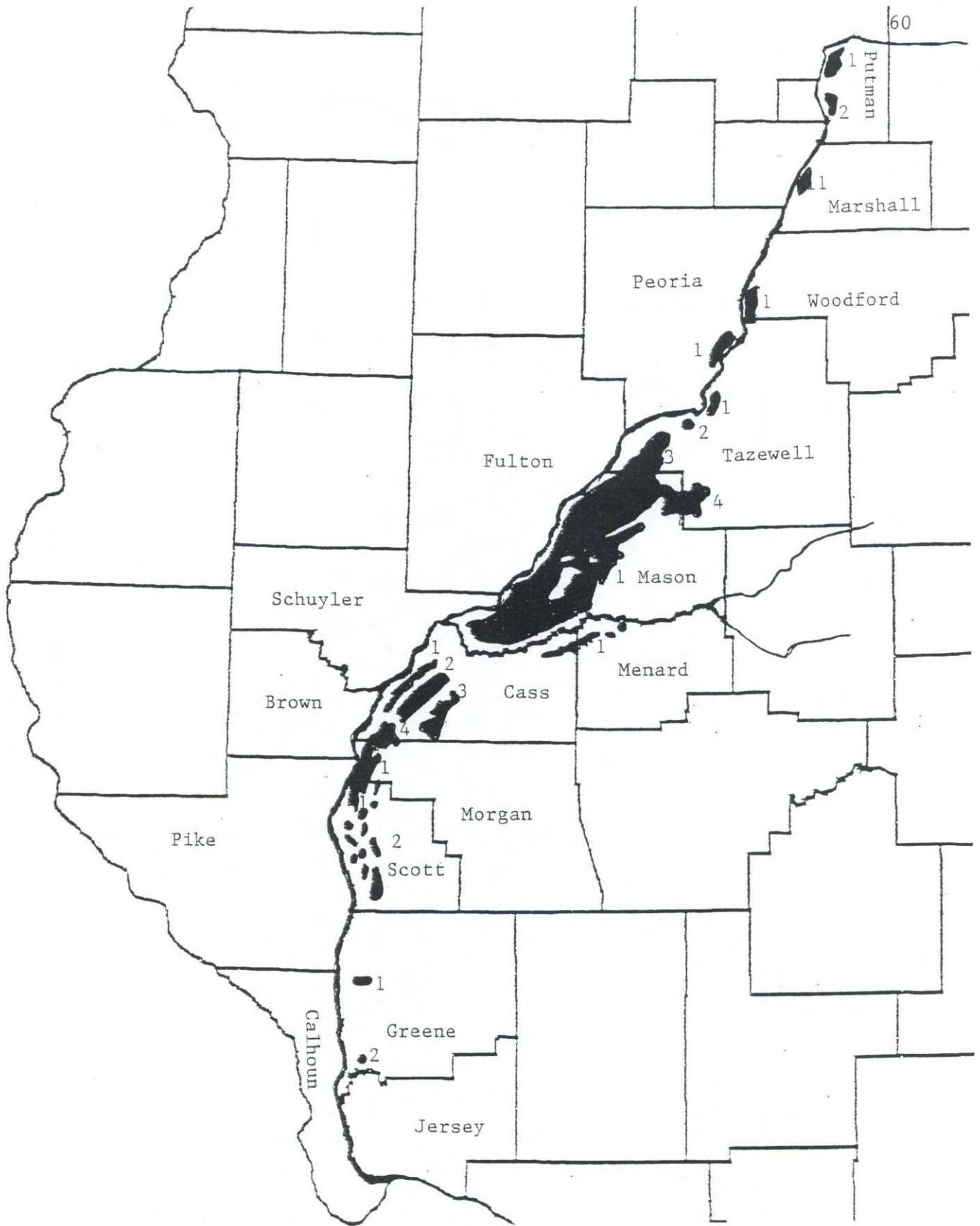
Figure 1. Map of the Illinois River valley from the "Big Bend" in Putnam County south to the Mississippi River with the distribution of the Illinois River sand deposits.
