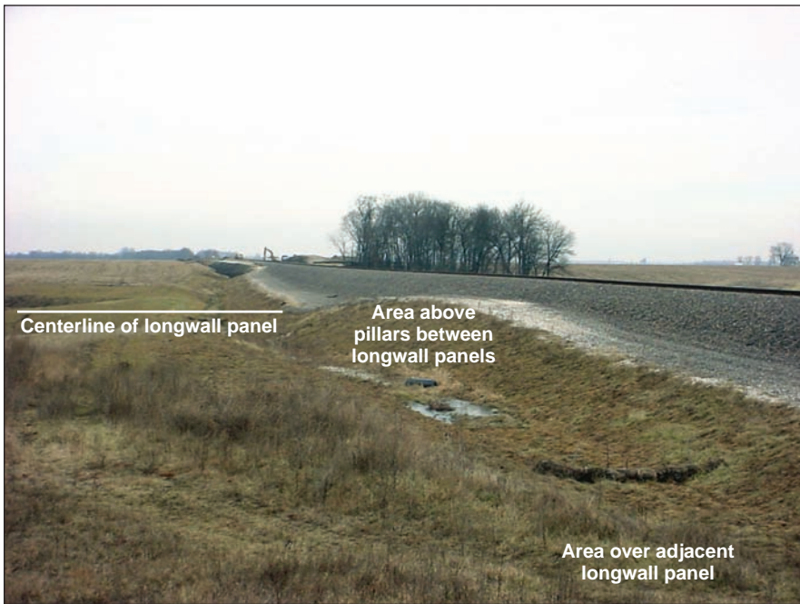
Figure 14 This railroad grade was re-established after longwall coal mine subsidence by increasing the vertical amount of crushed rock (ballast) below rails where longwall panels crossed under the tracks. (Photograph by Dan Barkley.)
