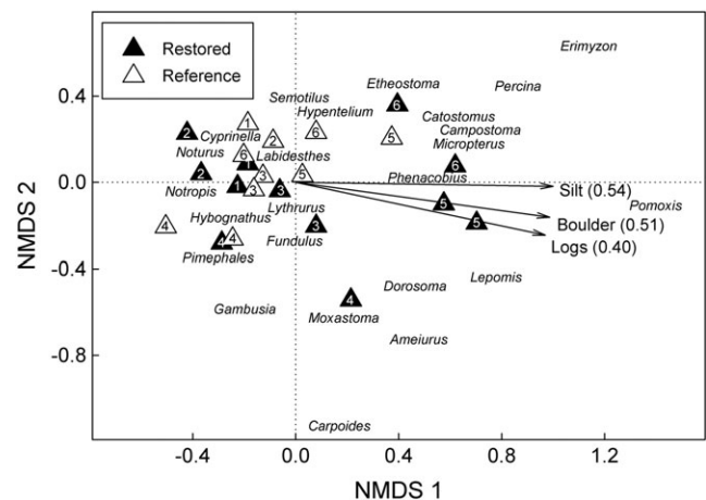
FIGURE 2 Nonmetric multidimensional scaling (NMDS) plot computed with a Bray–Curtis dissimilarity matrix examining temporal and spatial changes in community structure following an instream restoration project in Kickapoo Creek. Fish communities were sampled in restored and reference sites from 2010 to 2015 and numbers within the plot correspond to years post restoration (1–6). Relative loadings of taxonomic groups are represented by genera. Solid vectors represent significant ( \alpha < 0.01 ) habitat parameters, with direction and magnitude related to the correlation to the community matrix. Habitat vectors are labelled by variable, with respective permutational R^2 values
