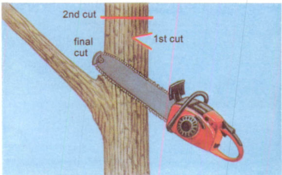
D. Crown reduction cut
