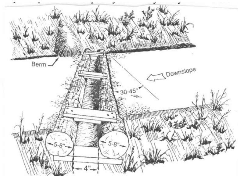
Figure 5-10. Open-top log culvert.
