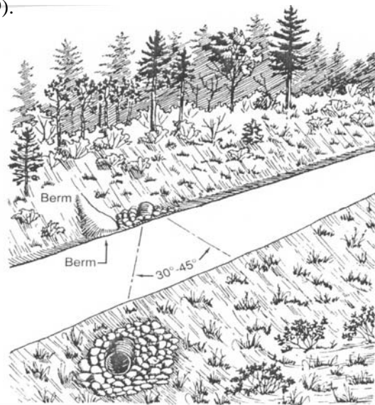
Figure 5-9. Cross-drain culvert.
