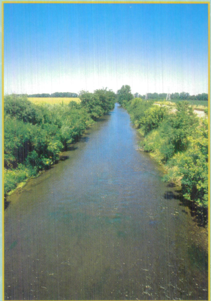
Channelized Stream
