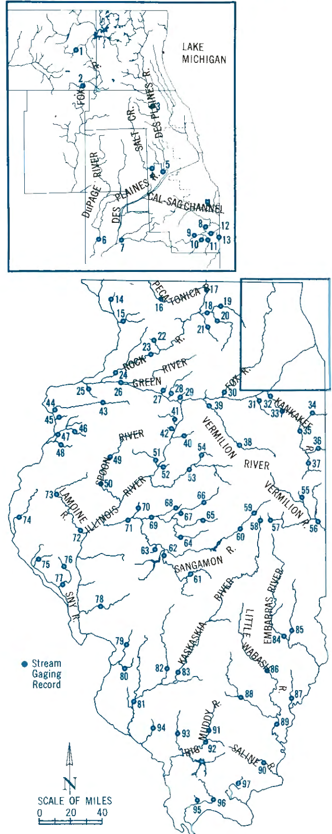
FIGURE 20 LOCATION OF STREAM GAGING STATIONS IN ILLINOIS
