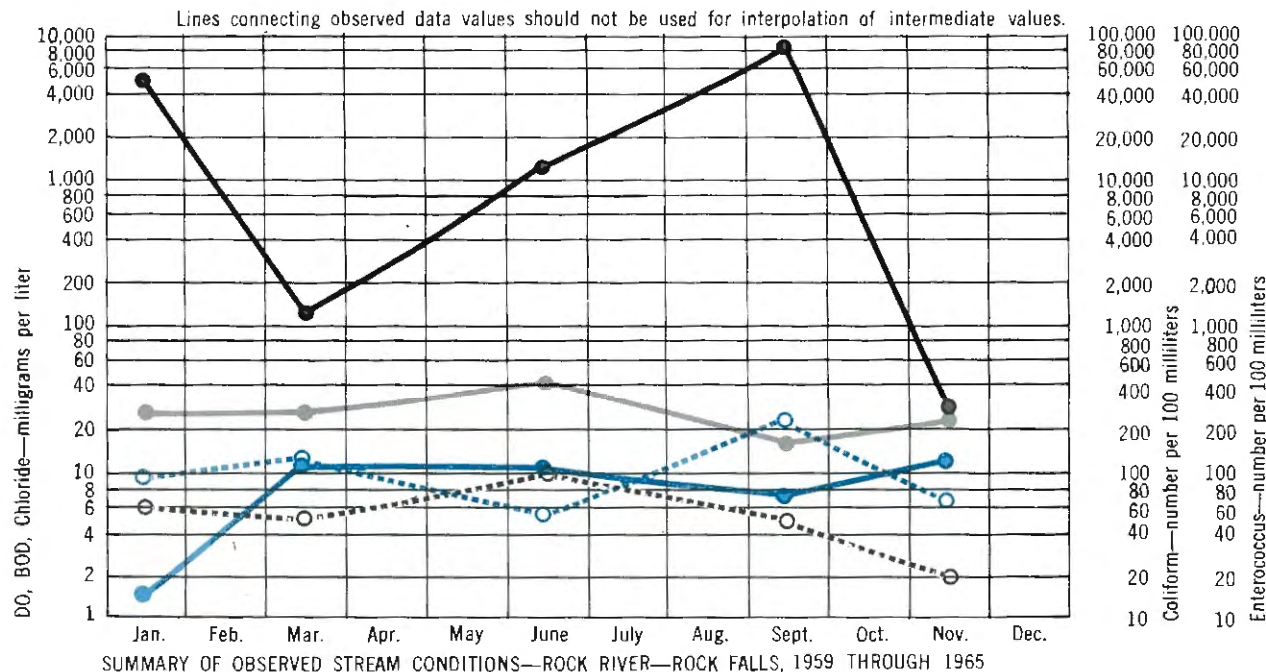
SUMMARY OF OBSERVED STREAM CONDITIONS—ROCK RIVER—ROCK FALLS, 1959 THROUGH 1965
